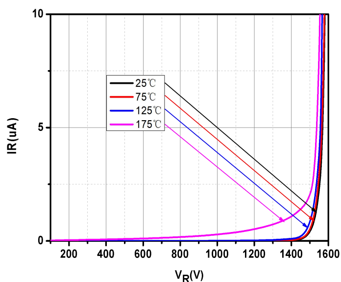
Fig.2-Typical Reverse Characteristics
