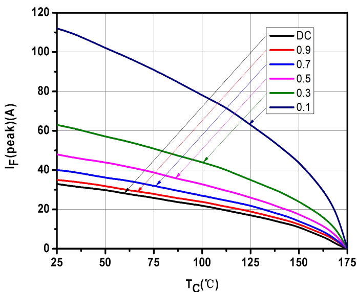
Fig.4-Current Derating
